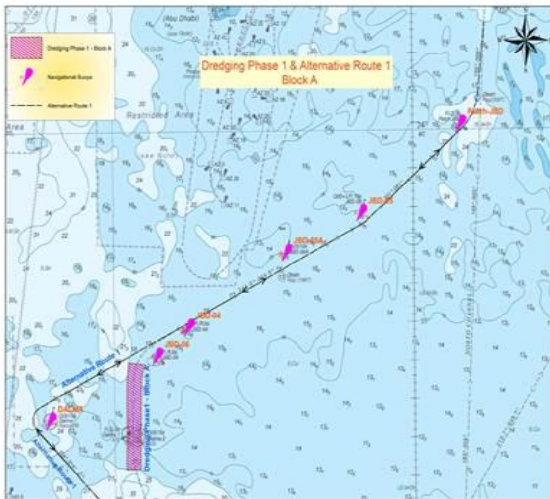
Figure 2. Dredging Phase - 1 Widening and deepening Block A
