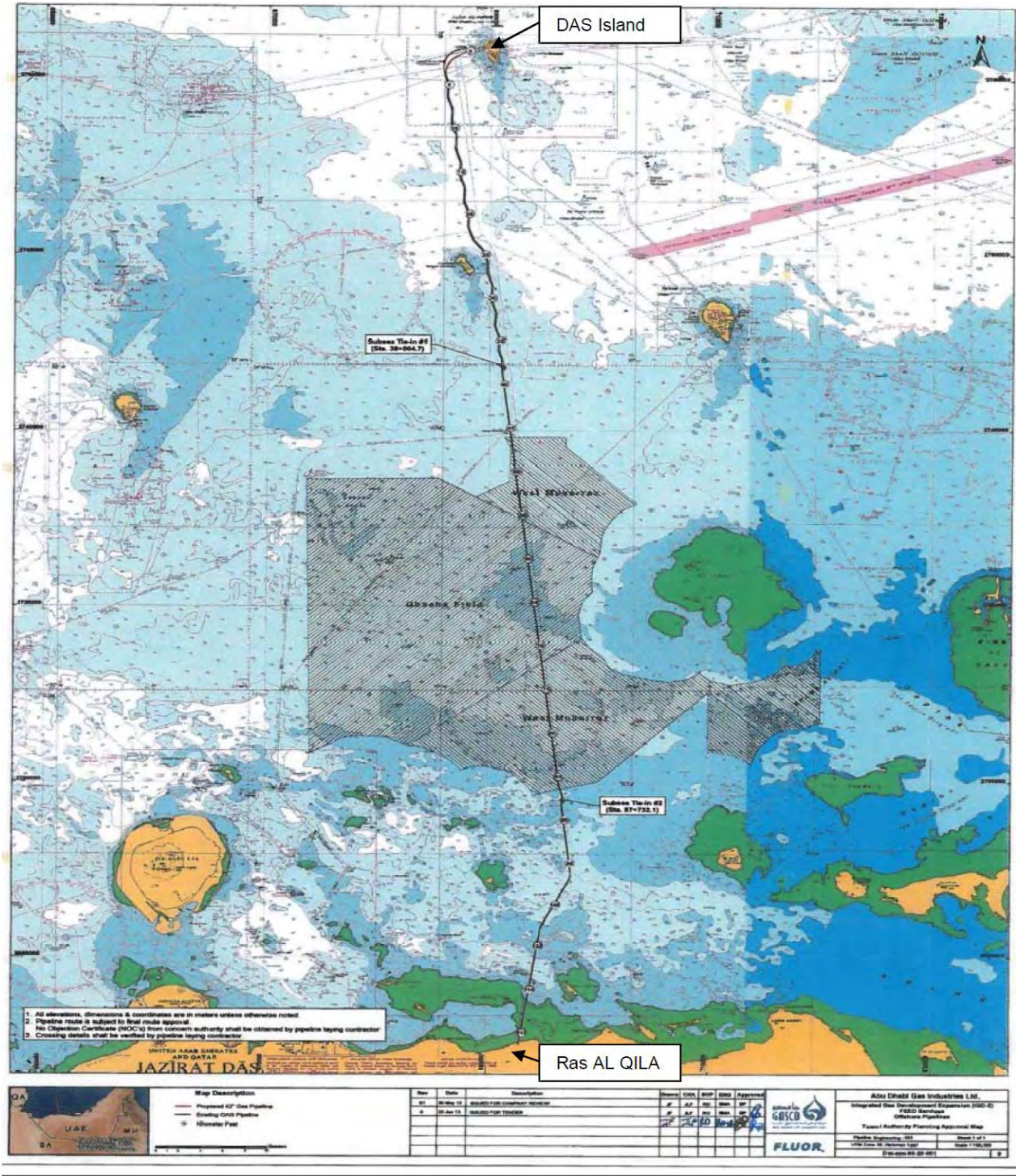
Figure 2: Proposed 42" IGD-E Pipeline Route Diagram
